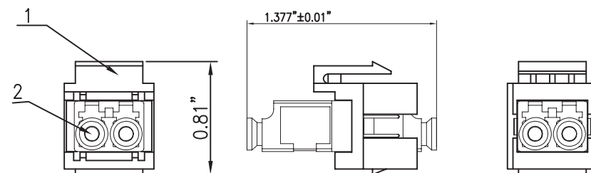
Assembly drawing
