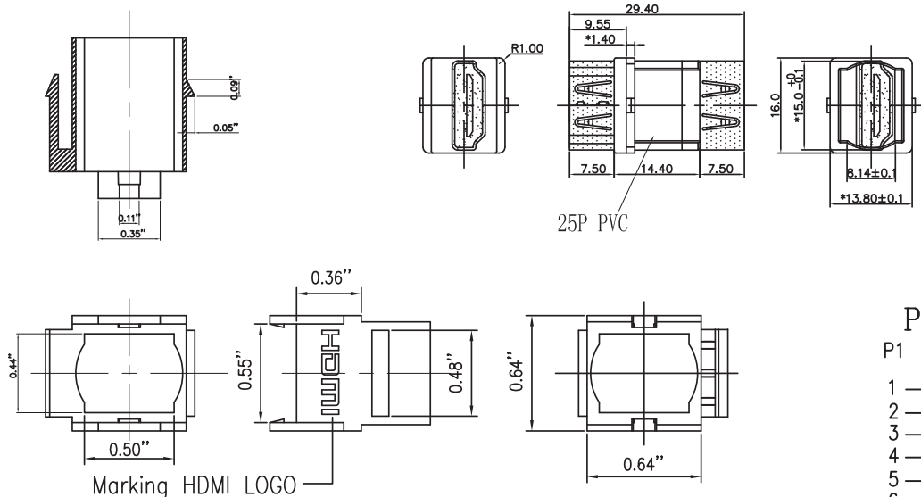
MODULE DRAWING(UNIT:INCH)
