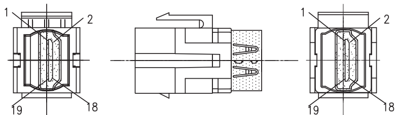
MODULE DRAWING(UNIT:INCH)
