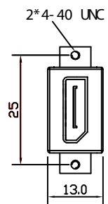
DisplayPort female
